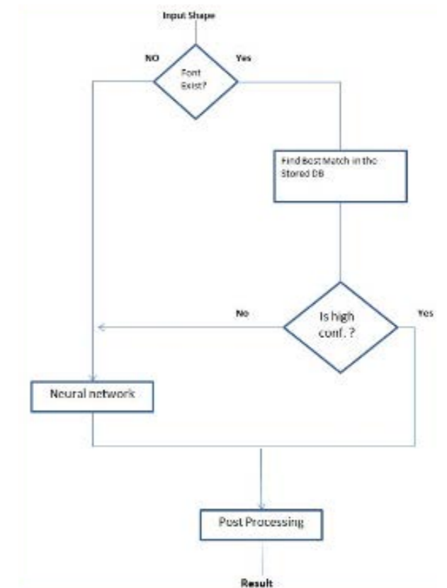
Figure 03 Arabic Text Recognition flow
